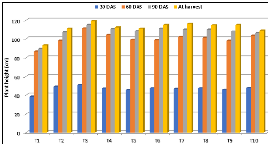
Fig 2: Effect of organic manures and inorganic fertilizers on plant height of wheat crop
